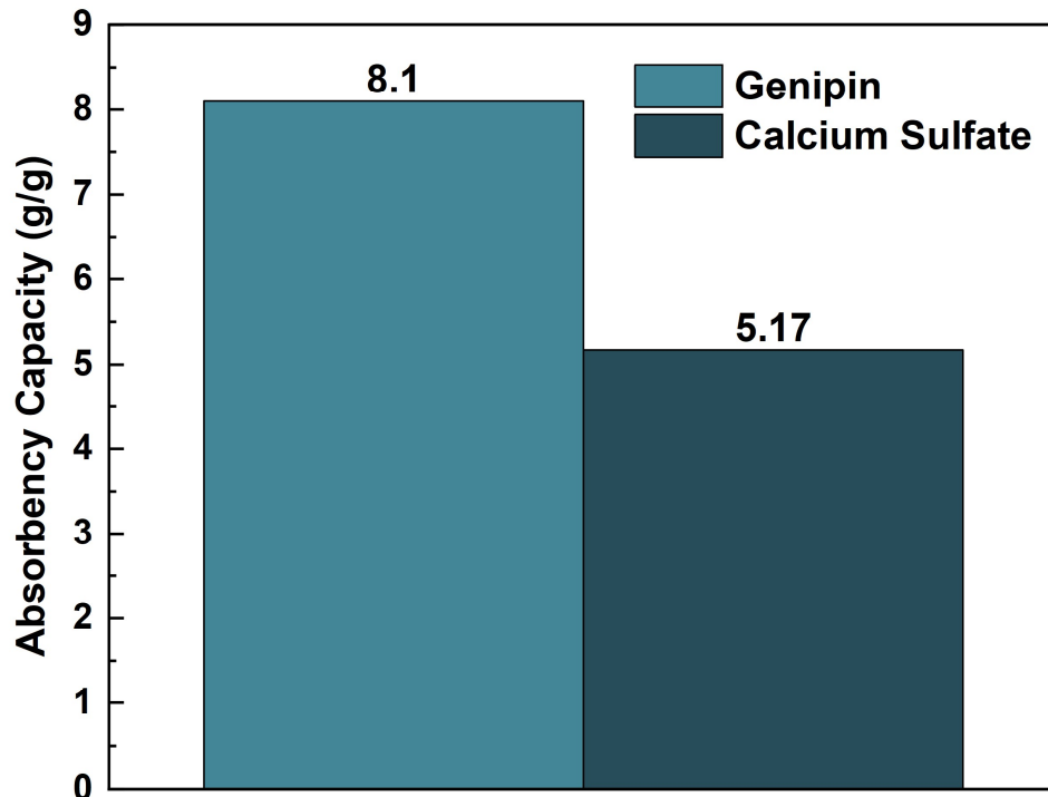
Figure 2- Comparison of the two crosslinkers, genipin and calcium sulfate, used to assess the absorbency capacity with sodium alginate.
