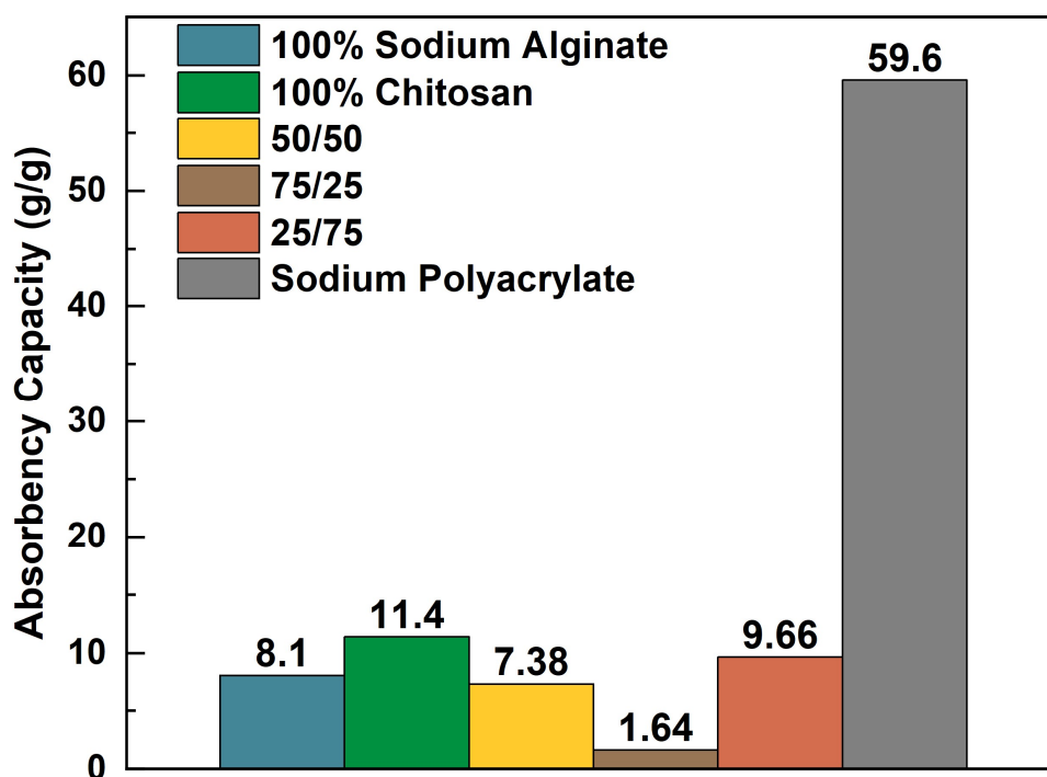
Figure 1- Comparison of each hydrogel with varying backbone ratios of sodium alginate to chitosan and industrial-grade sodium polyacrylate.
